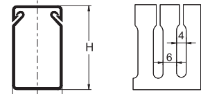
Slot Hole Size S=4mm
